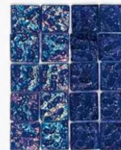
IRID Fernandina - Tephra
