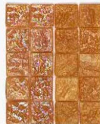
IRID Sundoro - Tephra
